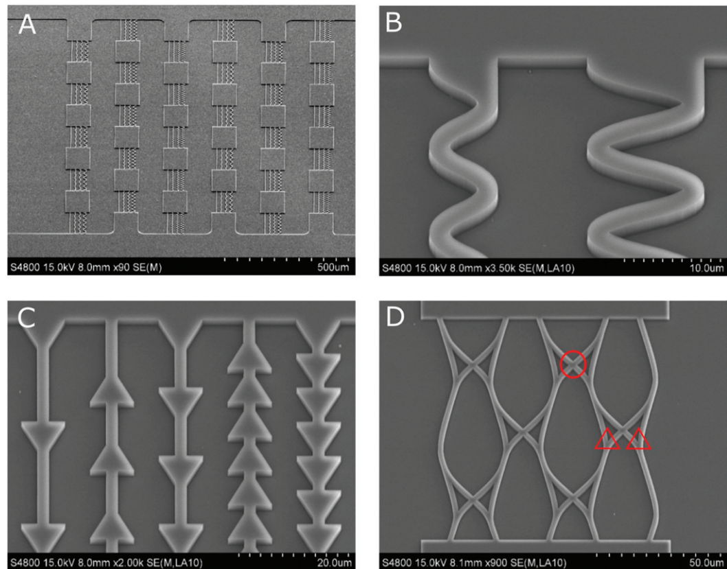
Figure 2. SEM graphs of monolithic Si casting master showing various test structures for 2 \mu\text{m} wide and 2 \mu\text{m} deep channels, obtained using a chlorine ICP system. (A) An overview of lines and curves/waves patterns. (B) Various curves. (C) Various arrows for rectifiers. (D) Pass junctions (indicated by the red circle) and split junctions (indicated by the red triangles).
